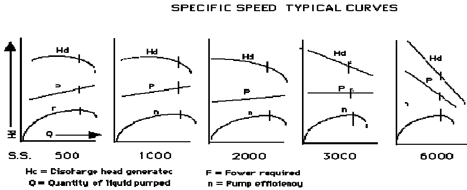
Fig. 2 Head vs. Specific Speed [10]
