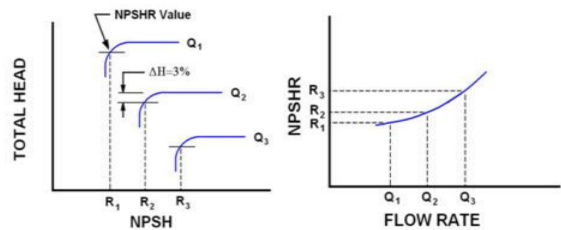
Fig. 14 NPSH_R Curve [21]
