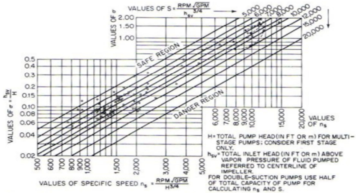
Fig. 13 Cavitation Regions [20]
